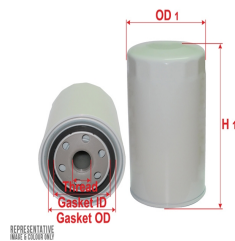
REPRESENTATIVE AC-51010 ES-12505
