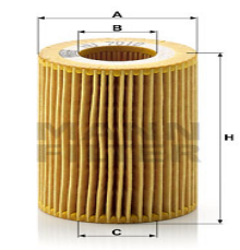
Oil Filter HU 7010 z EM-10127
