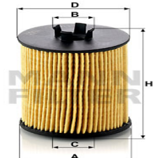
Oil Filter HU 612/1 x EM-10119
