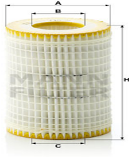
Oil Filter HU 718/5 x EM-10032
