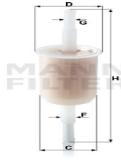
Fuel Filter WK 32 EM-20037
