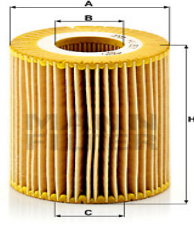
Oil Filter HU 821 x EM-10039
