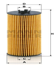
Oil Filter HU 6008 z EM-10125
