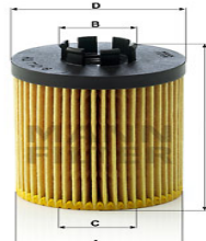
Oil Filter HU 712/8 x EM-10131
